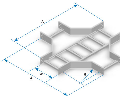
Diseño estructural para perfil "Z", "C" e "I" Segmented design for "Z", "C" & "I" rail type
