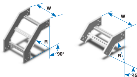
Diseño estructural para perfil "Z", "C" e "I" Segmented design for "Z", "C" & "I" rail type
